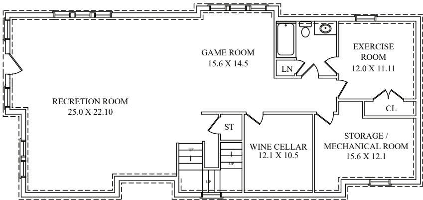
LOWER LEVEL
