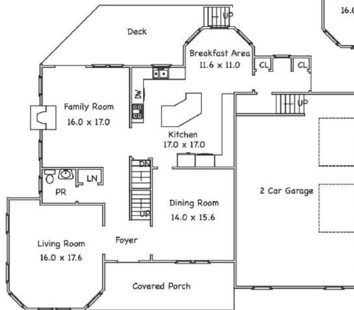
FIRST LEVEL
